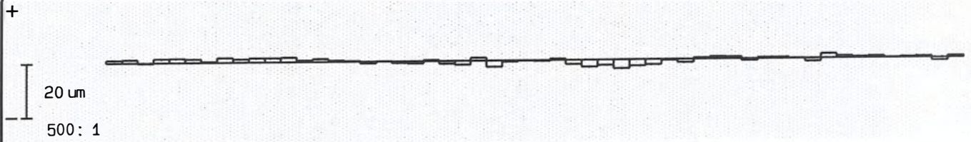
Tooth to Tooth Accumulative Fpi, Left Side (convex, Tooth)
