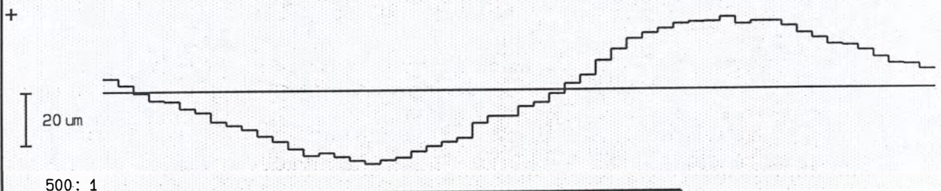
Runout Test
